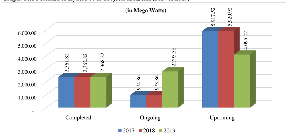
Graph: 16.1 Potential of Hydel Power Projects in AJ&amp;K (2017 to 2019)
